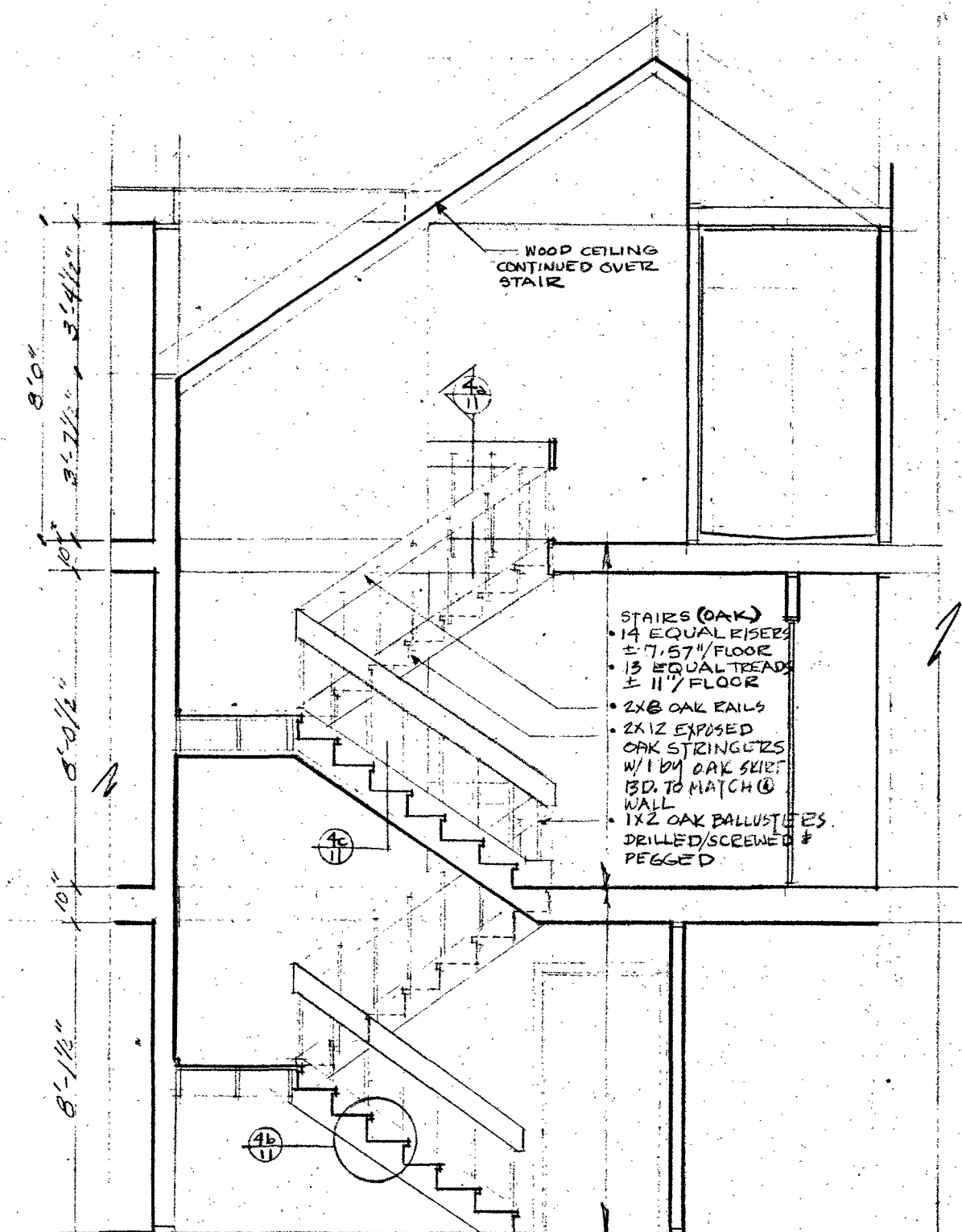
3 SECTION
