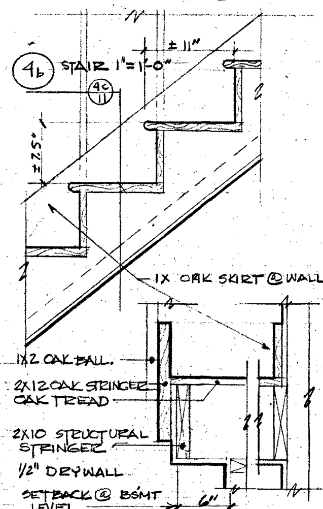
4b STAIR 1"=1'-0"
