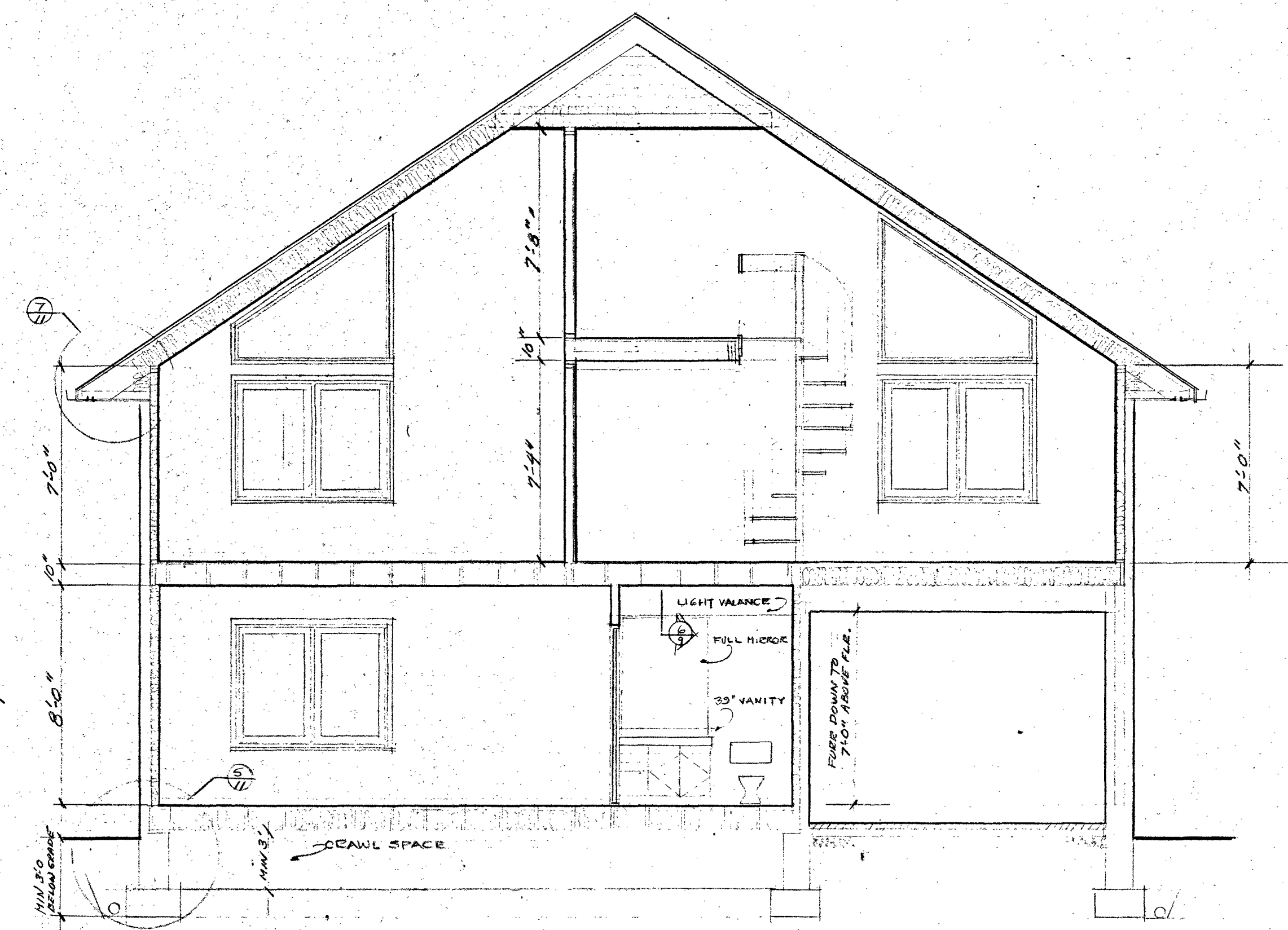
2 SECTION
