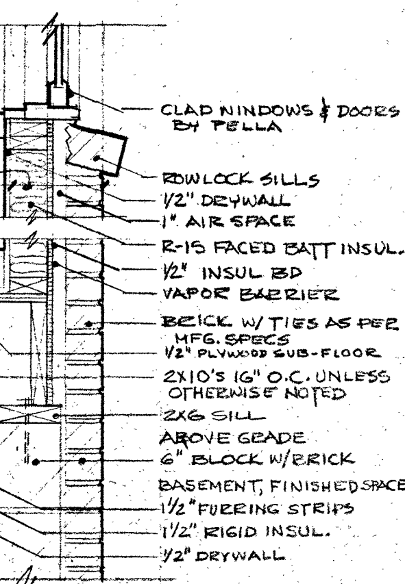
6 TYPICAL EXTERIOR WALL & WINDOW SILL 1"=1'-0"
