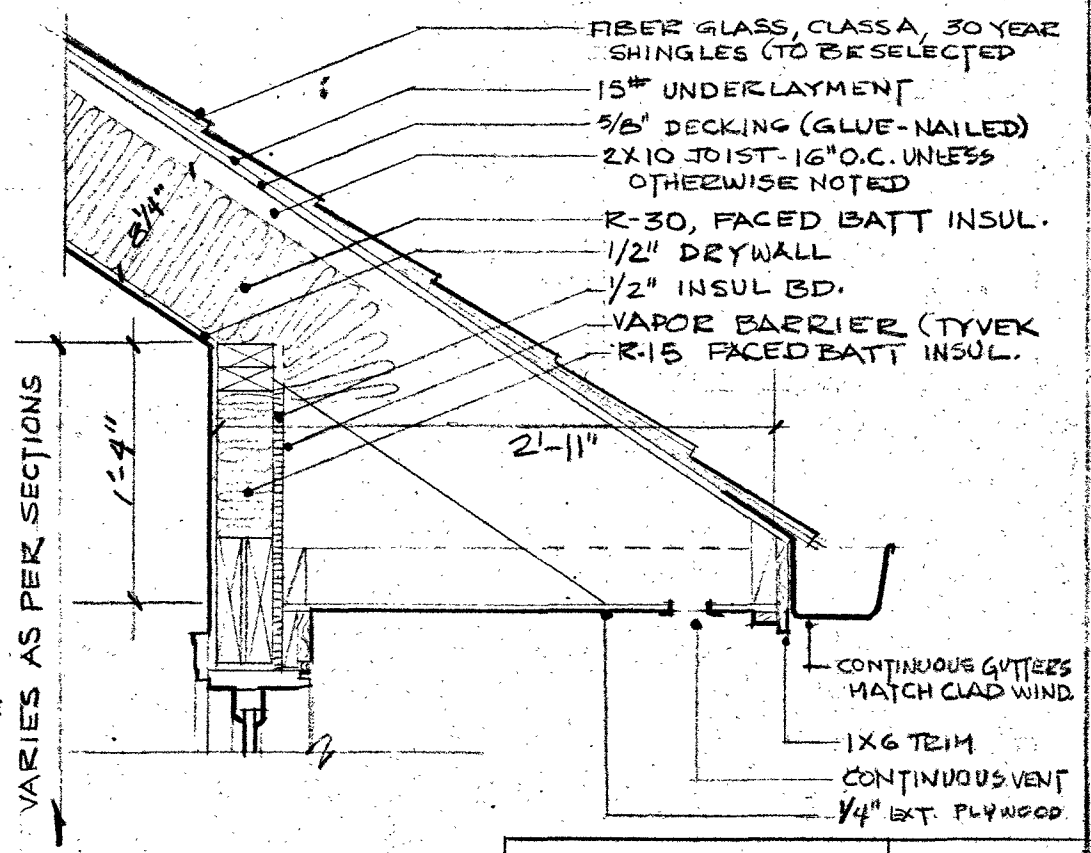
7 TYPICAL ROOF SOFFIT 1"=1'-0"
