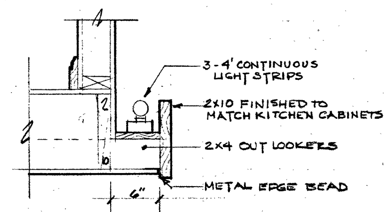
⑦ KITCHEN VALANCE LIGHT
