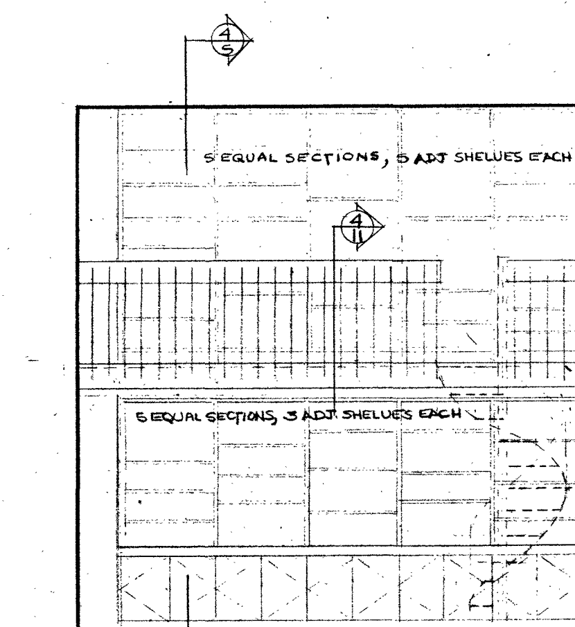
3 BALCONY ELEVATION SEE CASEWORK ALLOWANCE
