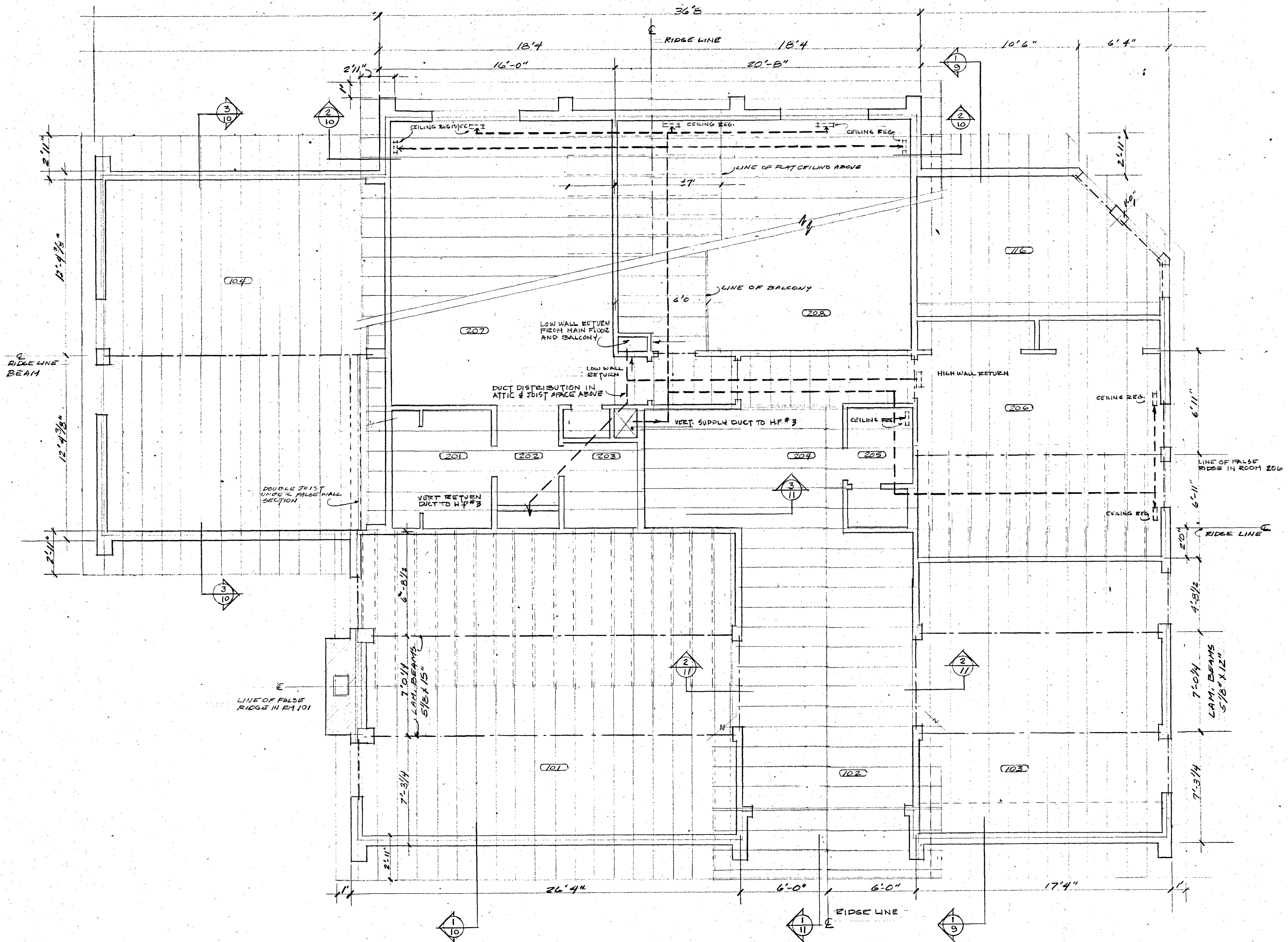
1 ROOF/CEILING FRAMING PLAN
