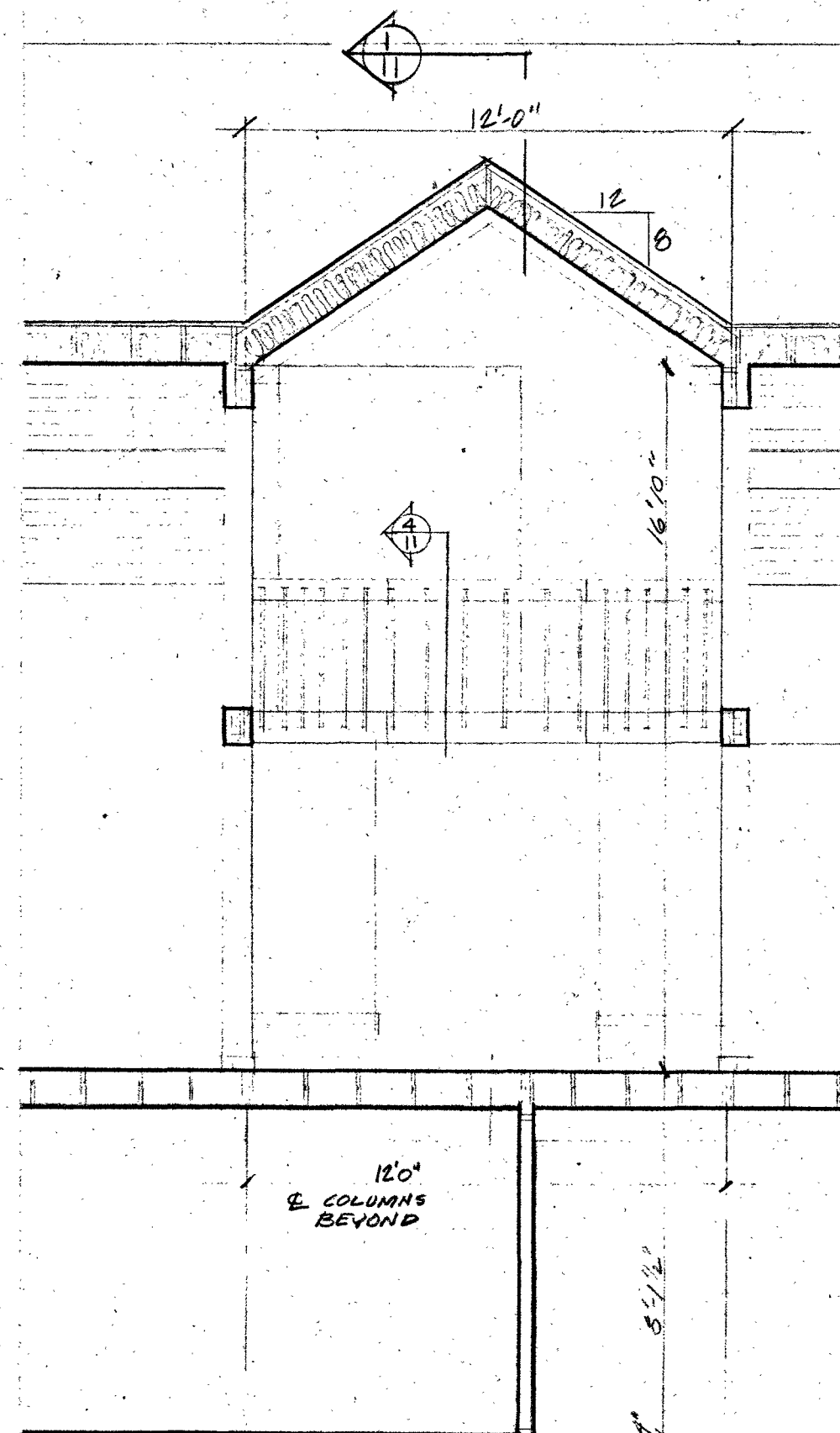
2 SECTION
