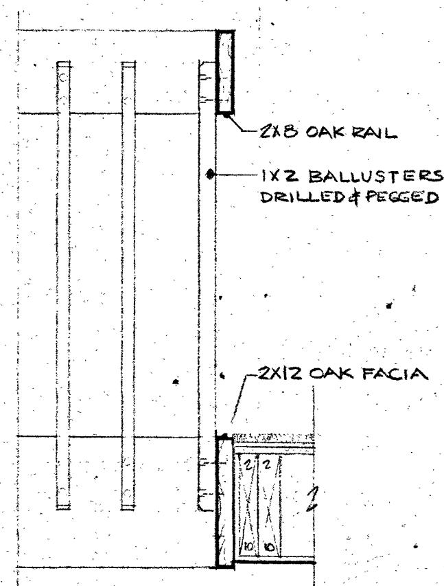
4a TYPICAL RAIL DETAIL 1"=1'-0"
