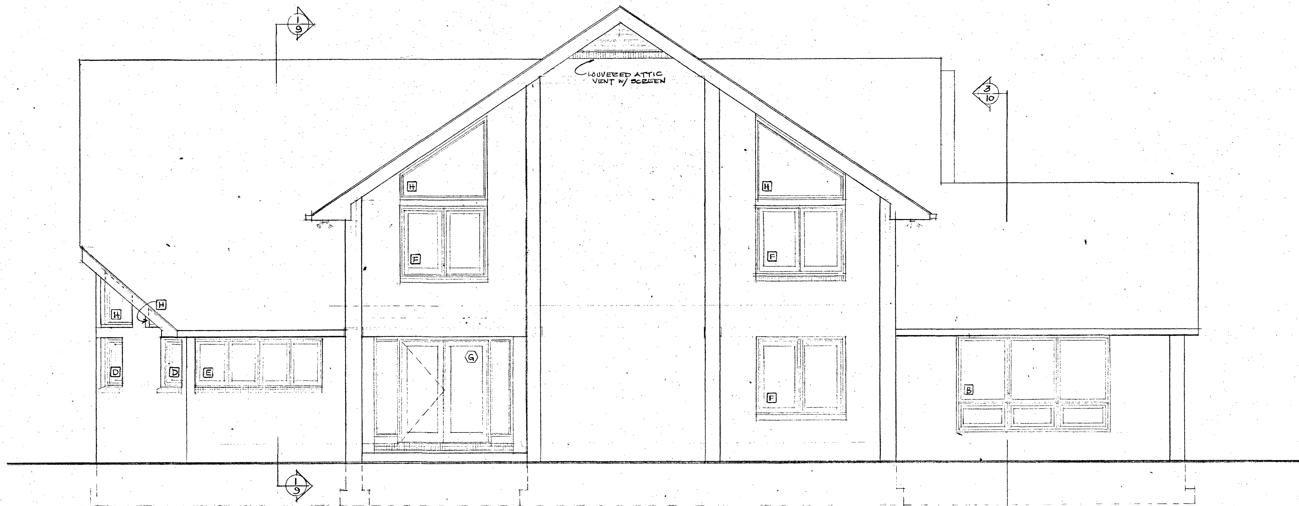
1 NORTH ELEVATION
