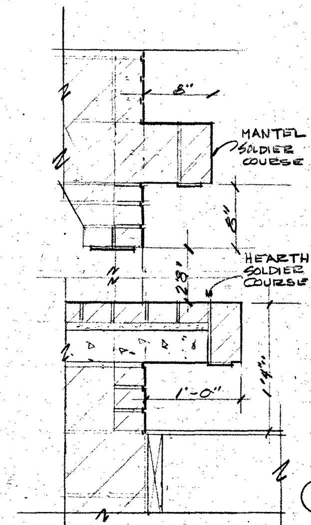
1 SECTION
