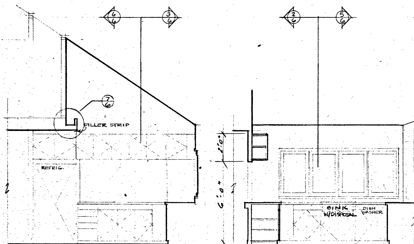
② KITCHEN ELEVATION/SECTIONS
