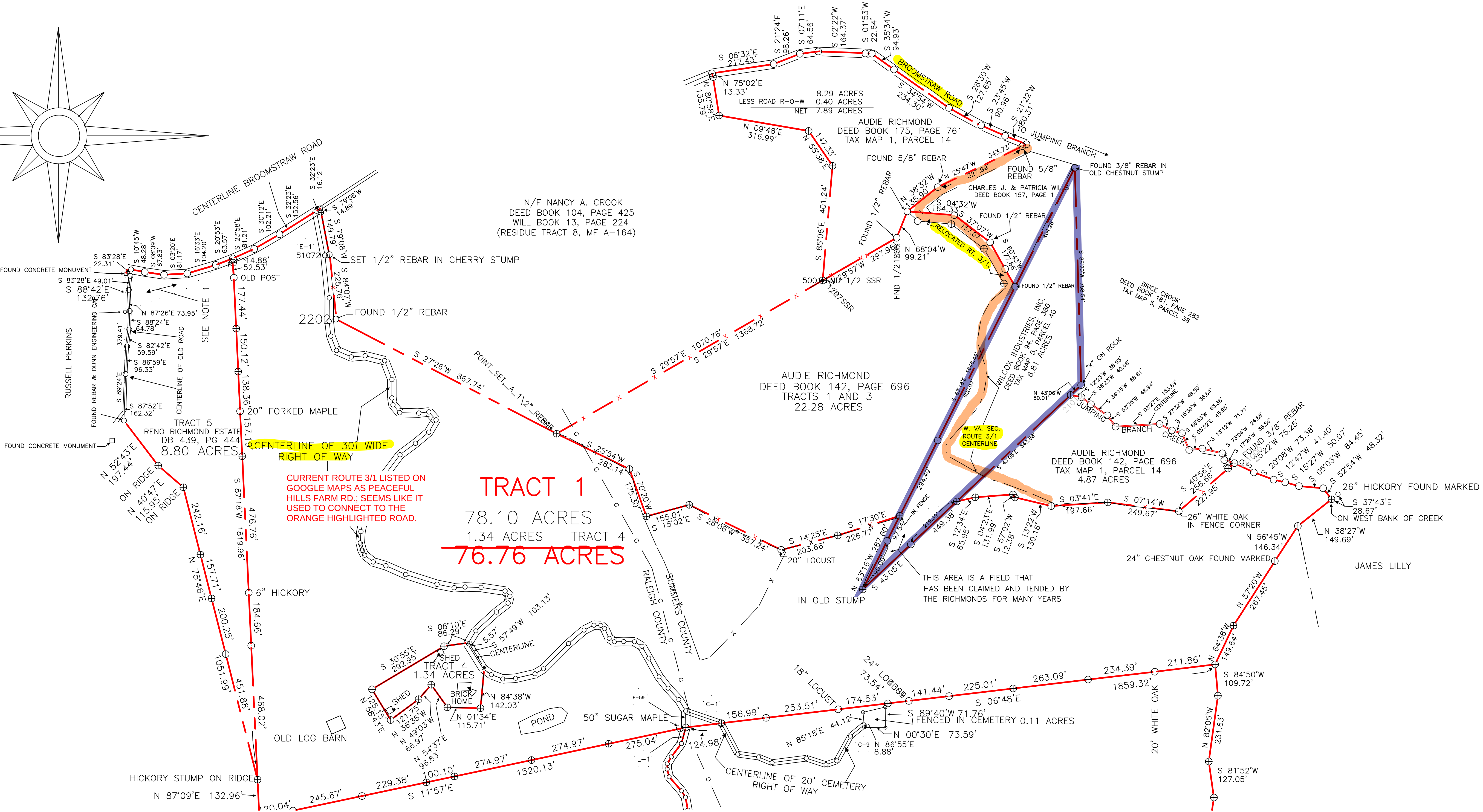
CENTERLINE OF 30' WIDE RIGHT OF WAY BETWEEN TRACT 2 & 3
