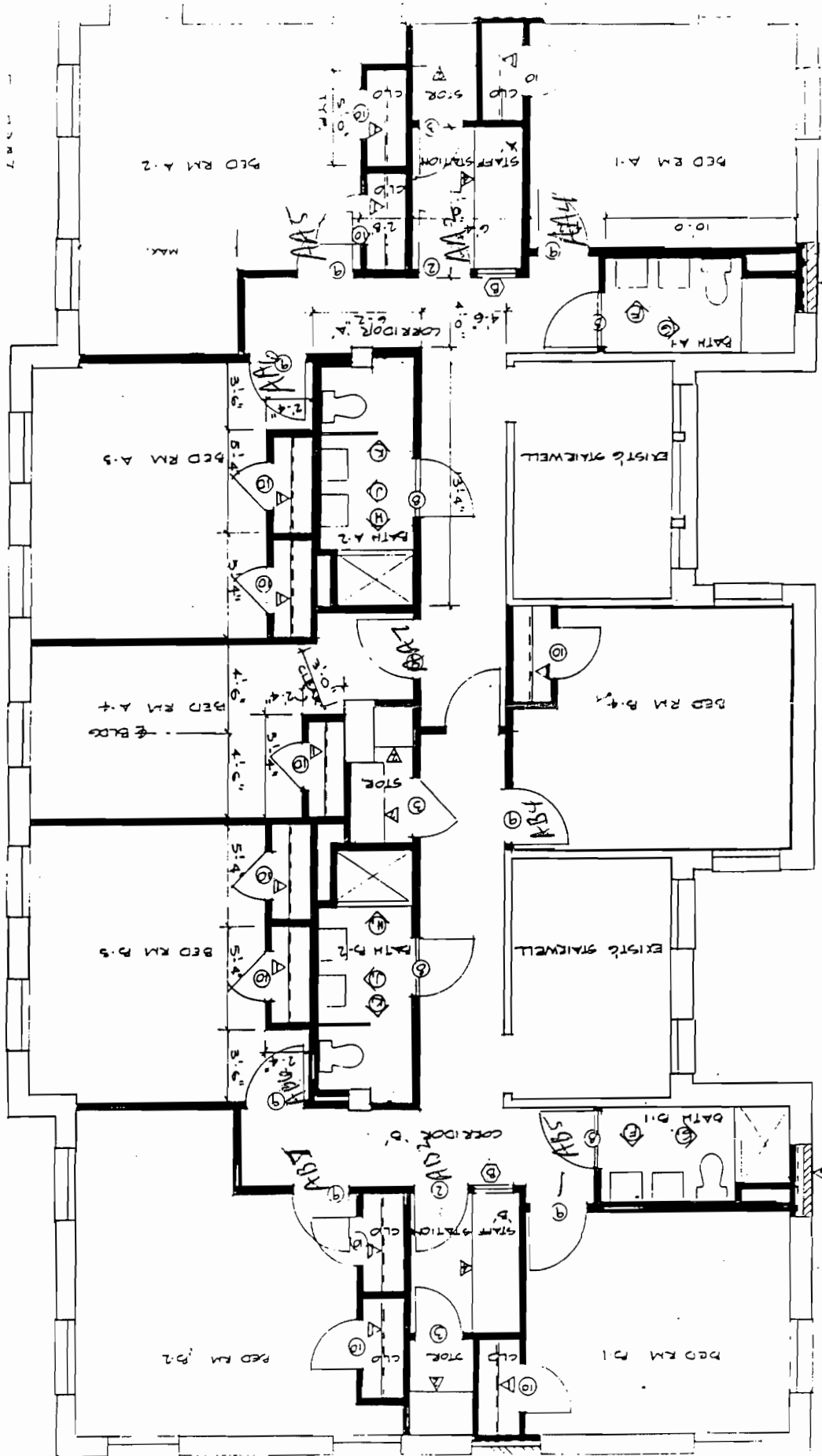
HUGHES MEMORIAL HOME TYPICAL RESIDENCE SECOND FLOOR 1/8" = 1'-0"
